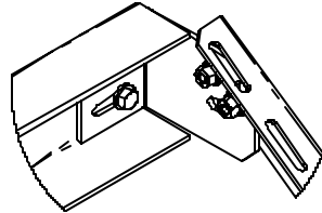
DETAIL B SCALE 1 : 5
