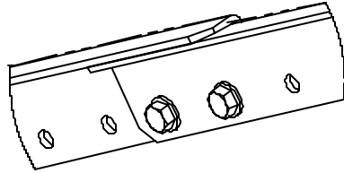
DETAIL C SCALE 1 : 3
